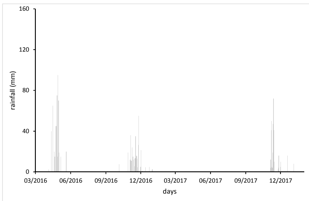
Fig. 2. Rainfall distribution during short rains 2016 and 2017
