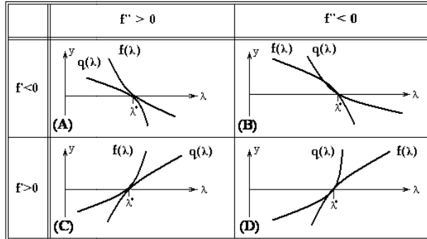
Fig. 1. Behavior of the functions f(\lambda) and q(\lambda) in the neighborhood of a simple real root \lambda^* of functions f(\lambda)
