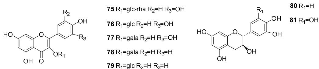
Fig. 3. Structures of selected flavonoids from L. formosana
