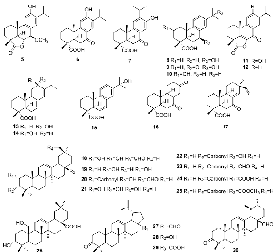
Fig. 2. Structures of selected diterpenes and triterpenoids from L. formosana
