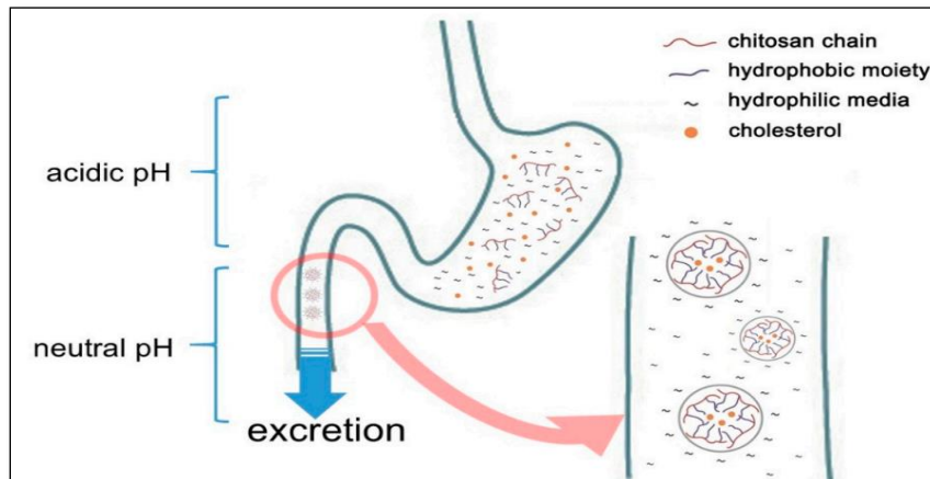
Fig. 3. Cholesterol adsorption of chitosan in gastrointestinal tracts [45]
