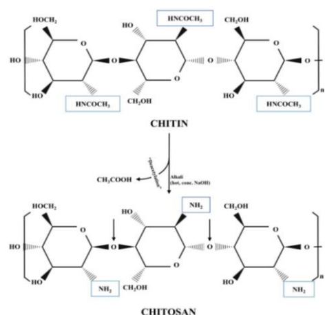
Fig. 1b. Deacetylation of chitin to produce chitosan [36]
